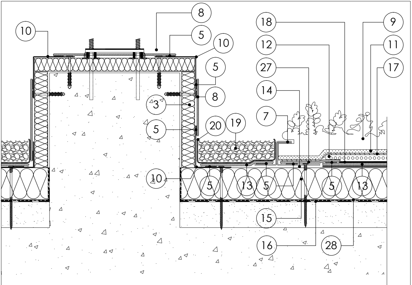
14.00 Plant Plinth Detail
