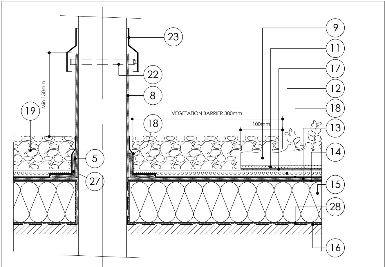
8.00 SVP Pipe Penetration Detail
